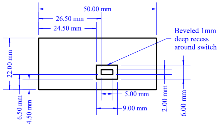
Right side Measurements NANOVNA V.2
