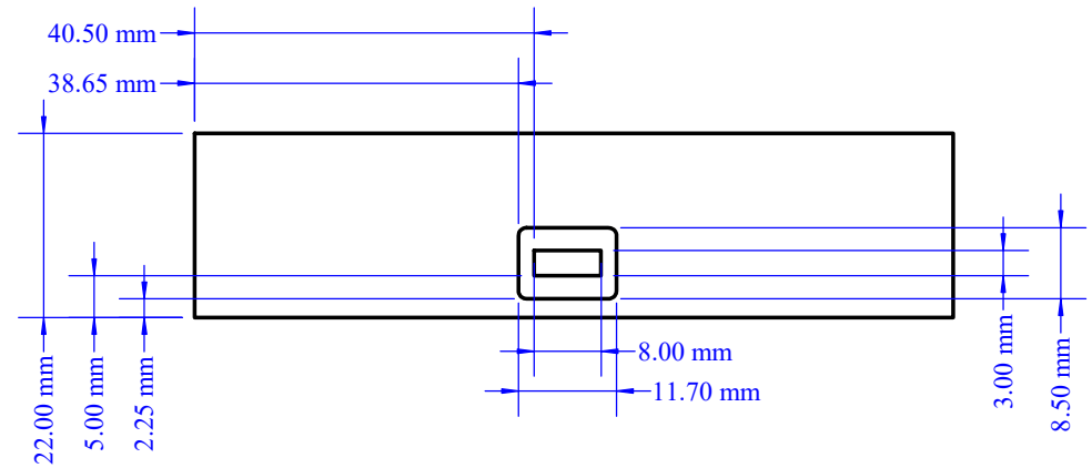
Bottom side Measurements NANOVNA V.2
